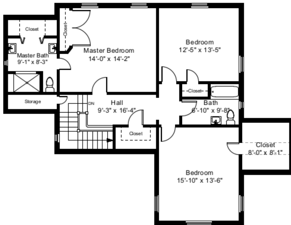
Second Floor Plan Ceiling Height = 8'-0"
